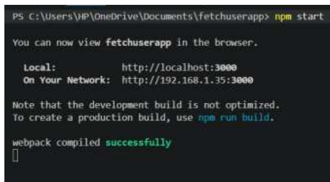
Figure 3: Terminal output
